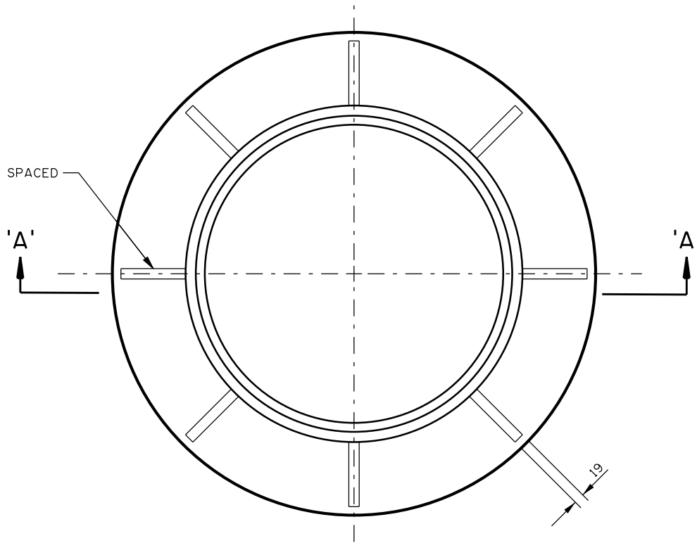
PLAN
