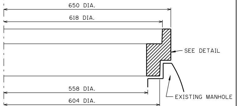
HALF SECTION
