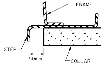
STEP DETAIL
