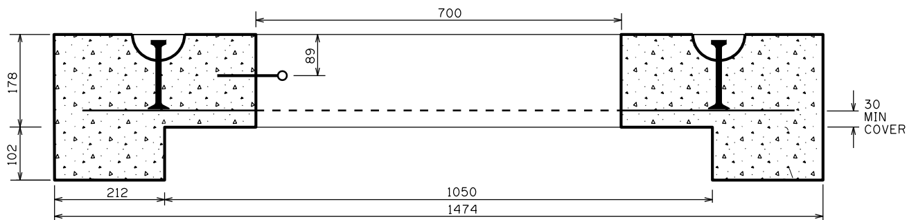
SECTION VIEW
