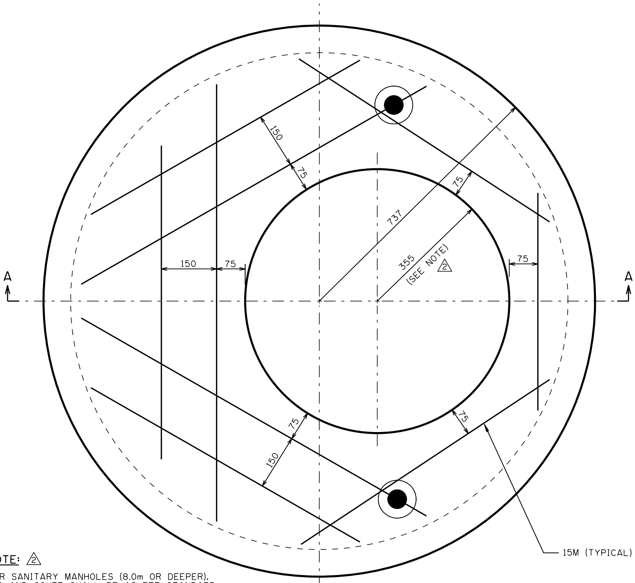
PLAN
