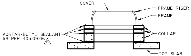
COLLAR DETAIL
