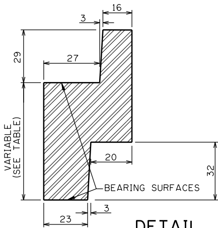
DETAIL
