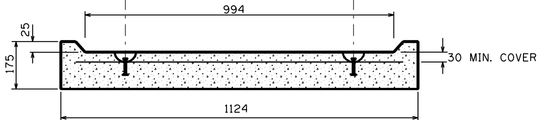
SECTION
