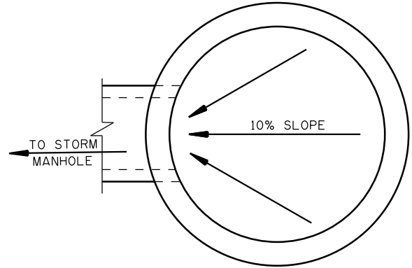
PLAN OF BOTTOM SLAB
