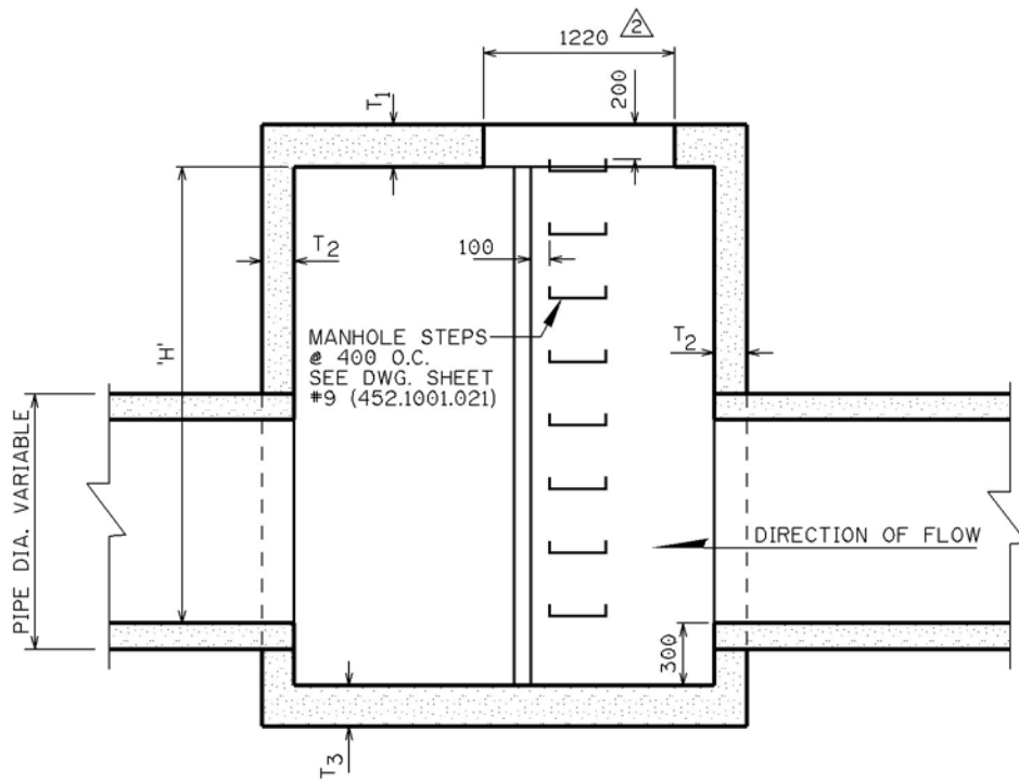
SECTION 'A-A'
