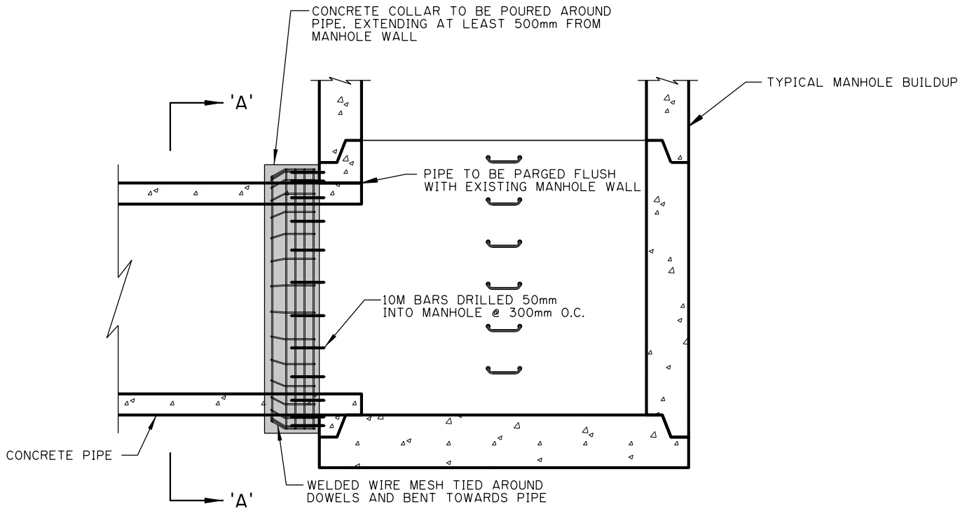
SECTION VIEW
