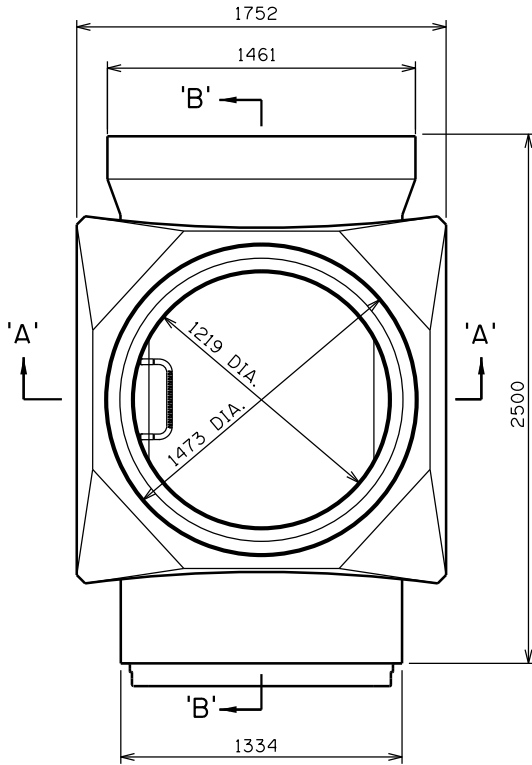
PLAN VIEW
