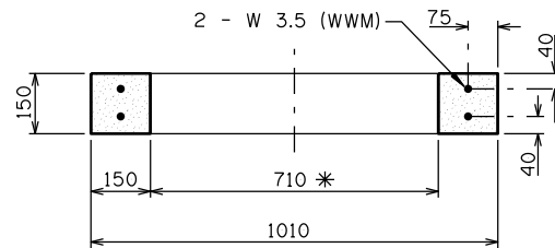
SECTION 150 COLLAR
