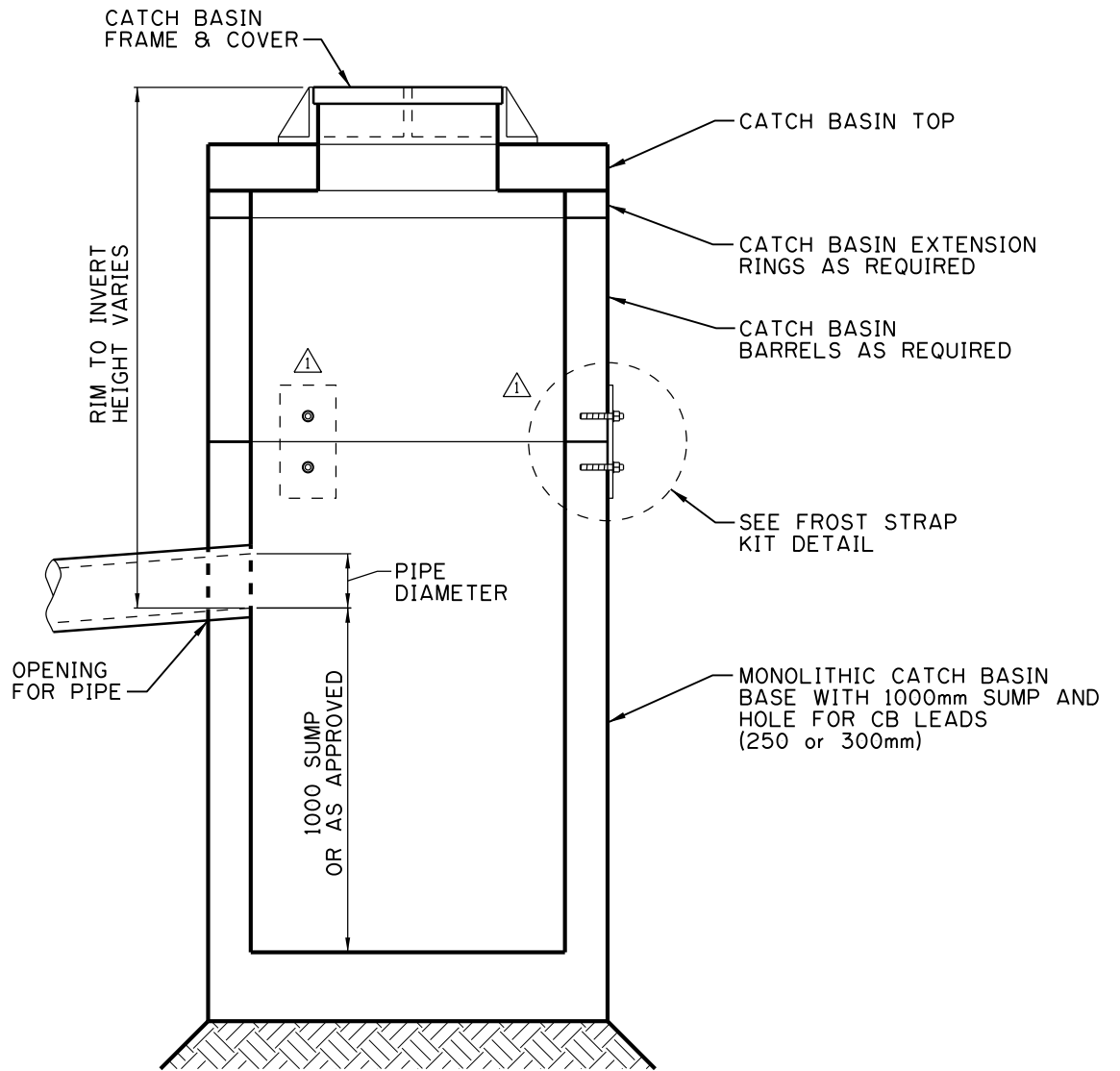
CATCH BASIN ASSEMBLY WITH 1000mm SUMP
