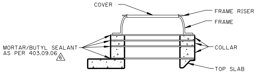
COLLAR DETAIL
