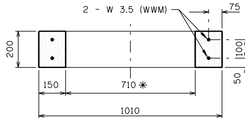
SECTION 200 COLLAR
