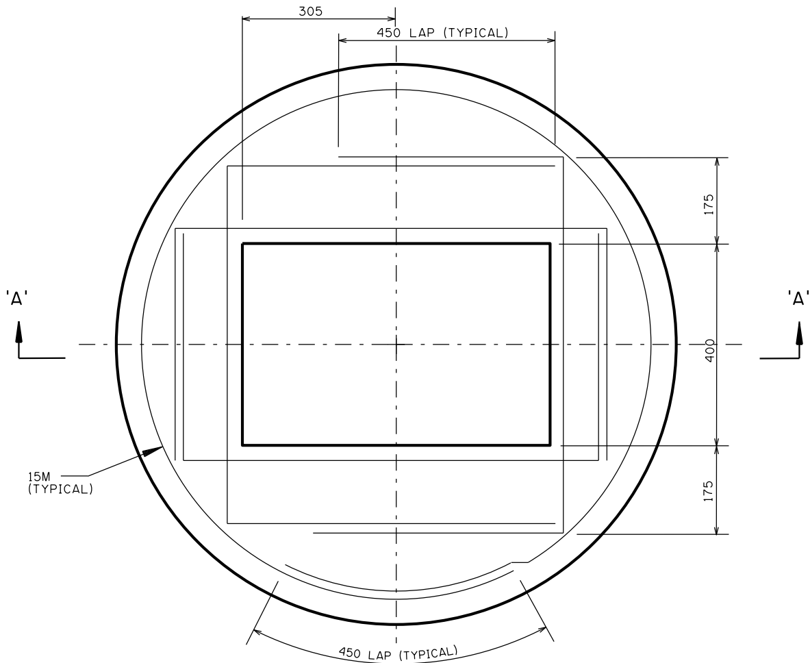
PLAN
