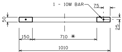
SECTION 50 COLLAR ⚠
