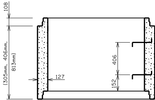
TOP BARREL
