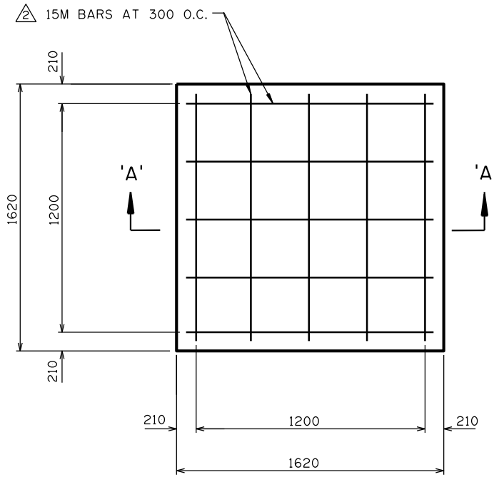
BASE SLAB
