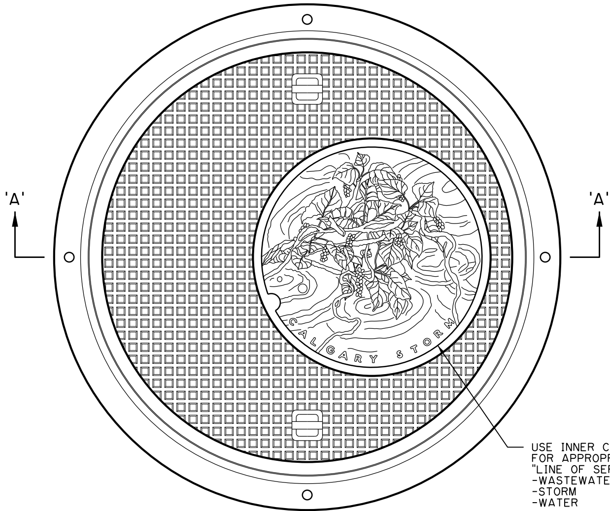
PLAN
