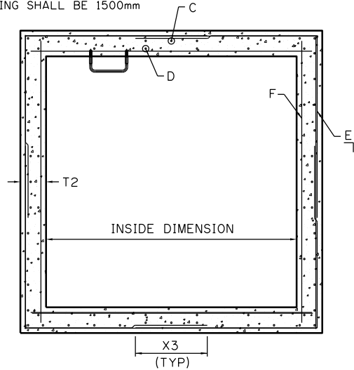
SECTION B
