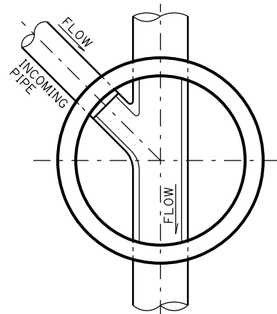
ALTERNATE (SEE NOTE 4)
