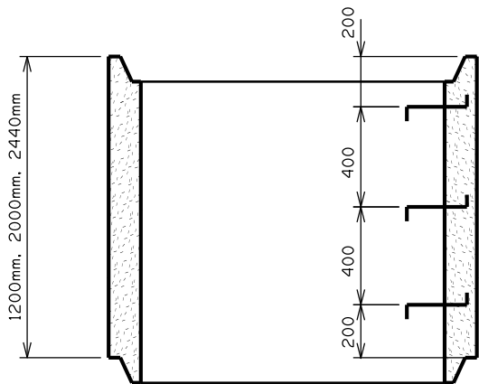
INTERMEDIATE BARREL SECTION 'A-A'
