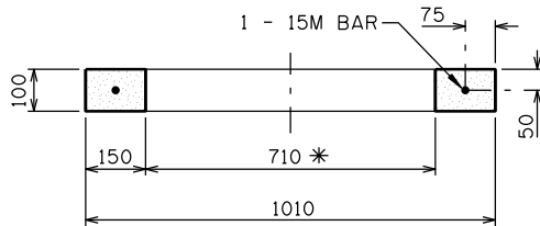
SECTION 100 COLLAR
