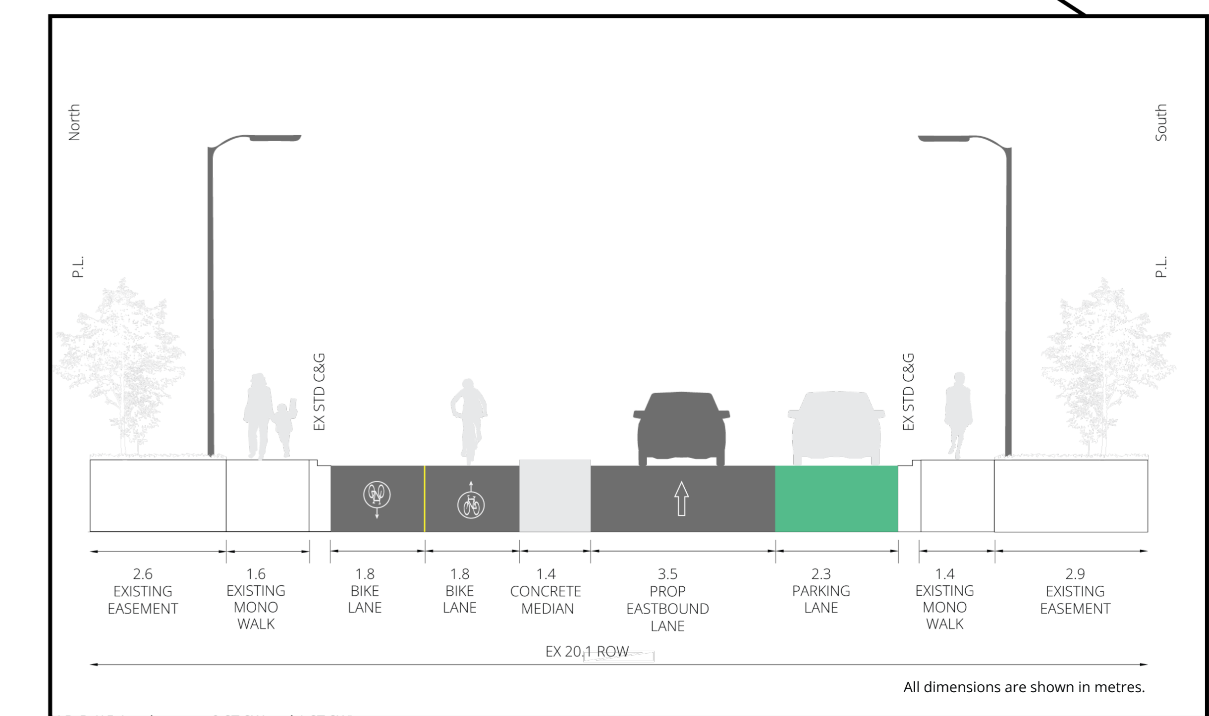
Cross Section D-D, 15 Avenue East of 2 Street SW
