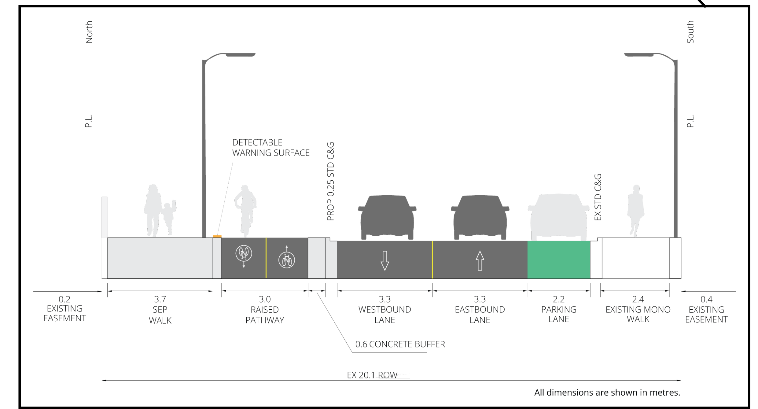
Cross Section E-E, 15 Avenue East of 1 Street S
