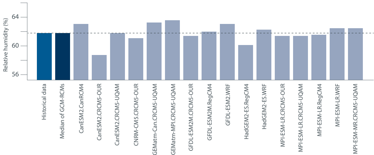
Figure 17. Comparison of relative humidity for current and 2050s future climate time series for the Calgary International Airport
